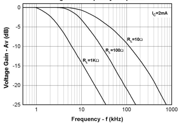
Figure 9. Frequency Response
